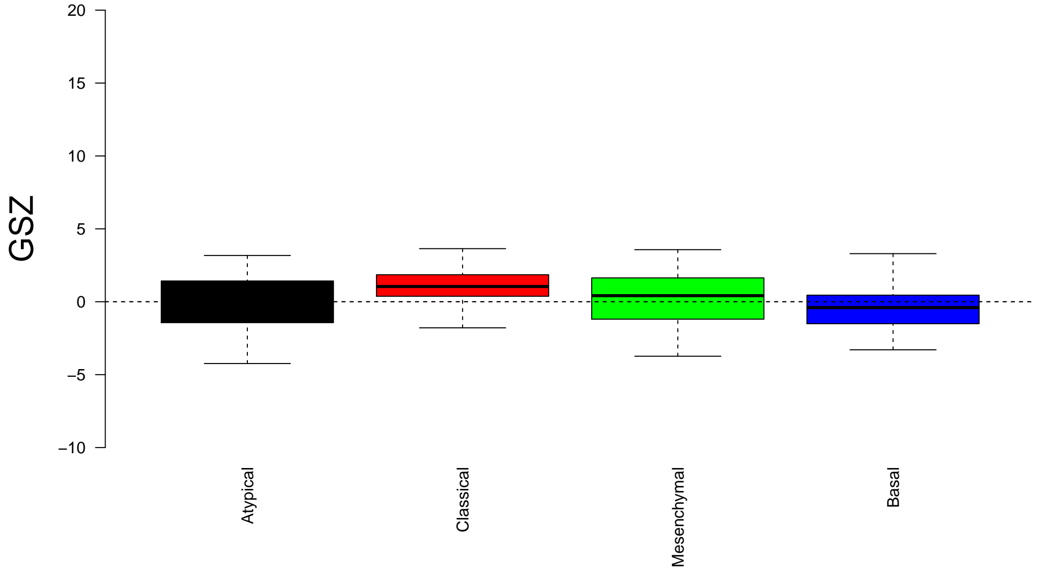
KUIPER_MM poor survival
